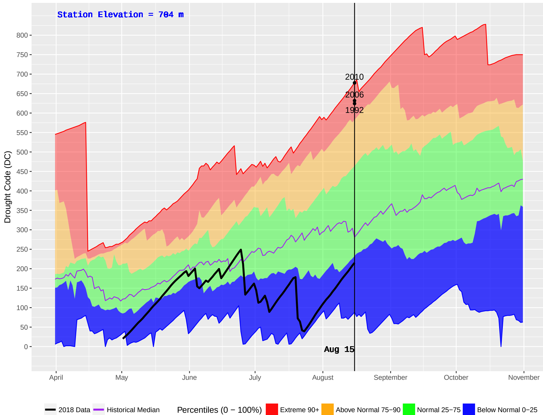
HUDSON HOPE (132) : Historical (1986–2016) and Current (2018) Daily Drought Code (DC)
