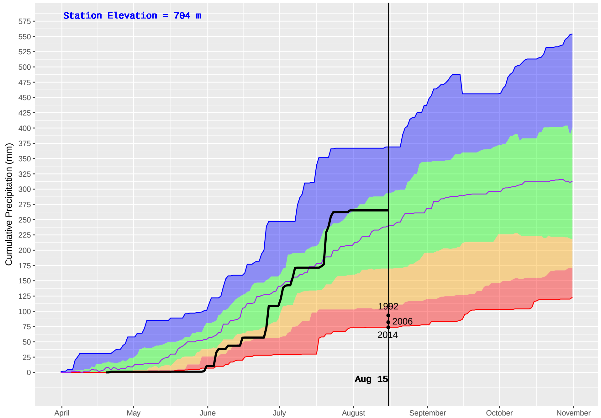
HUDSON HOPE (132) : Historical (1986–2016) and Current (2018) Daily Cumulative Precipitation
