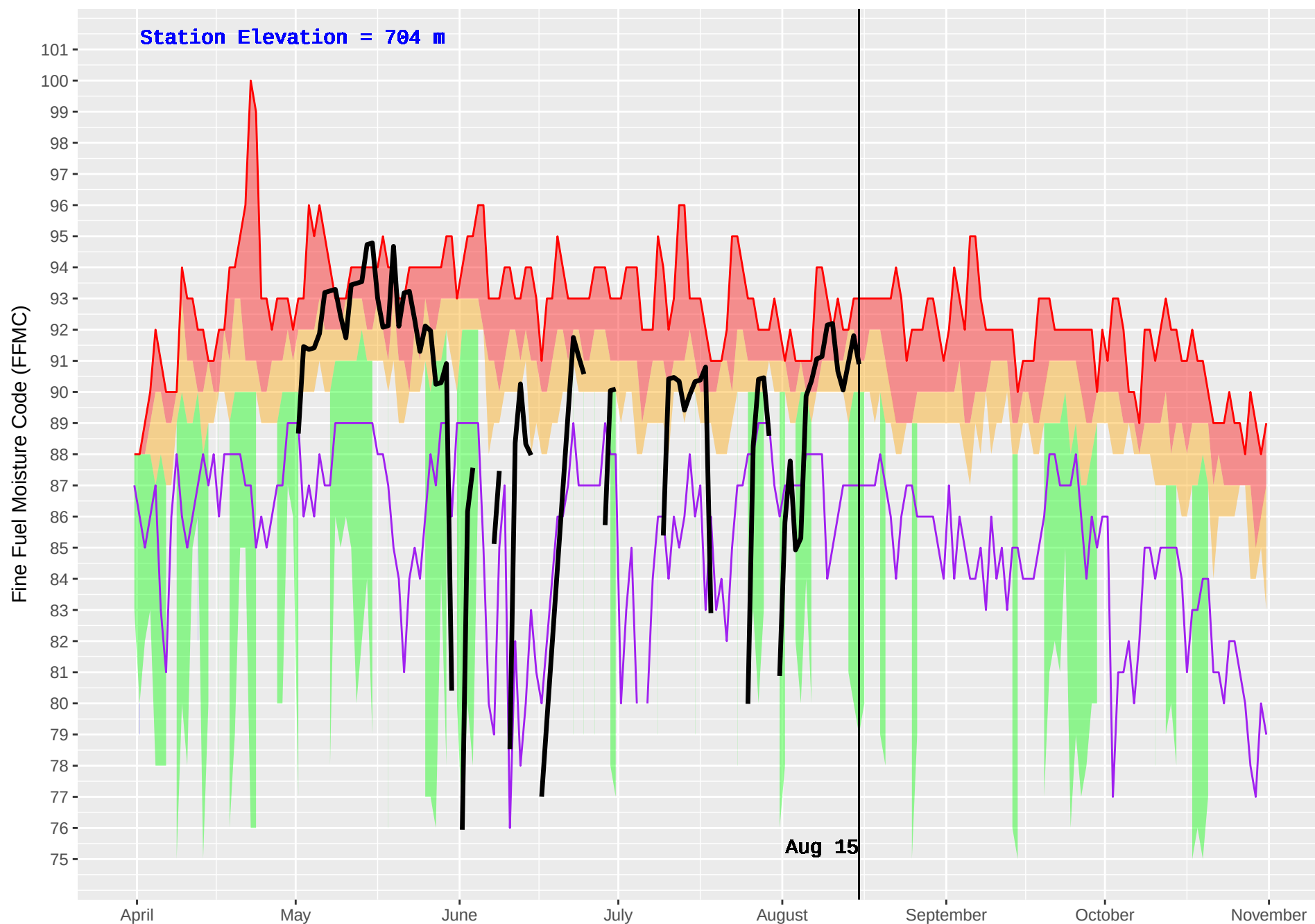
HUDSON HOPE (132) : Historical (1986–2016) and Current (2018) Daily Fine Fuel Moisture Code (FFMC)
